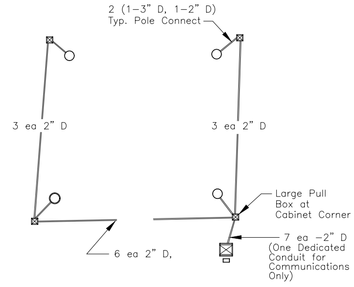
Conduit Detail – Typical 2" D. Schedule 80 PVC (Except as Noted)
