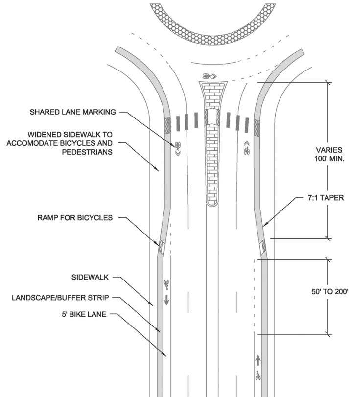
Figure 14-28 Multi-lane Roundabout
