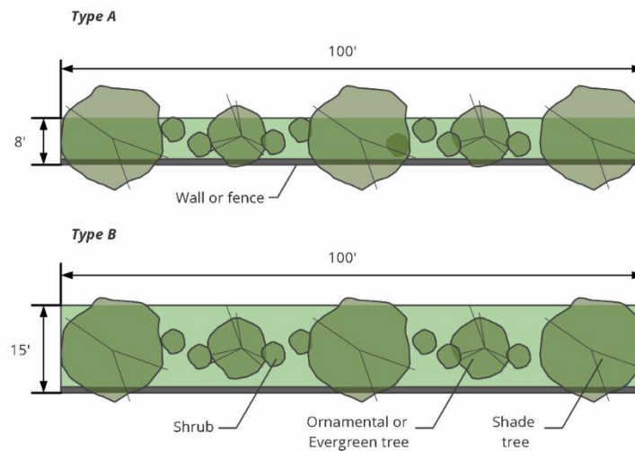
Figure 07.13-1 Buffer Requirements
