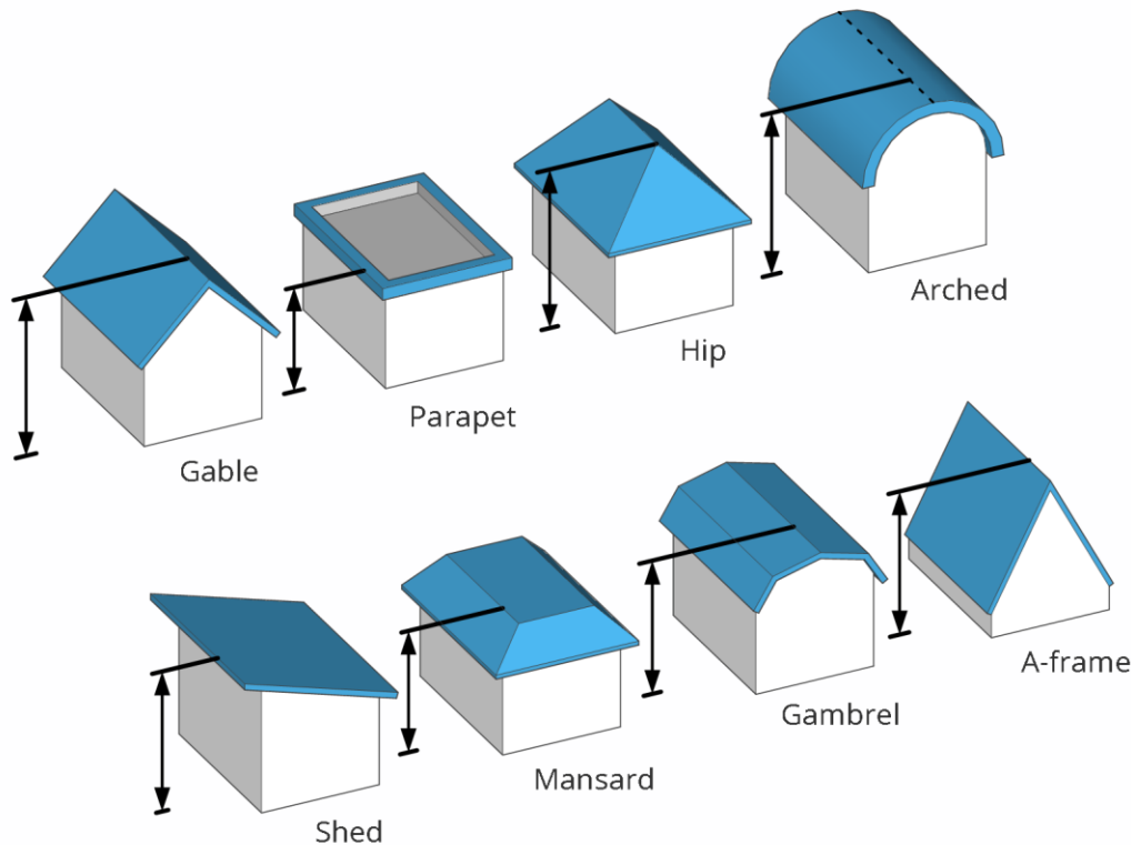
Figure 14.01-2 Roof Height
