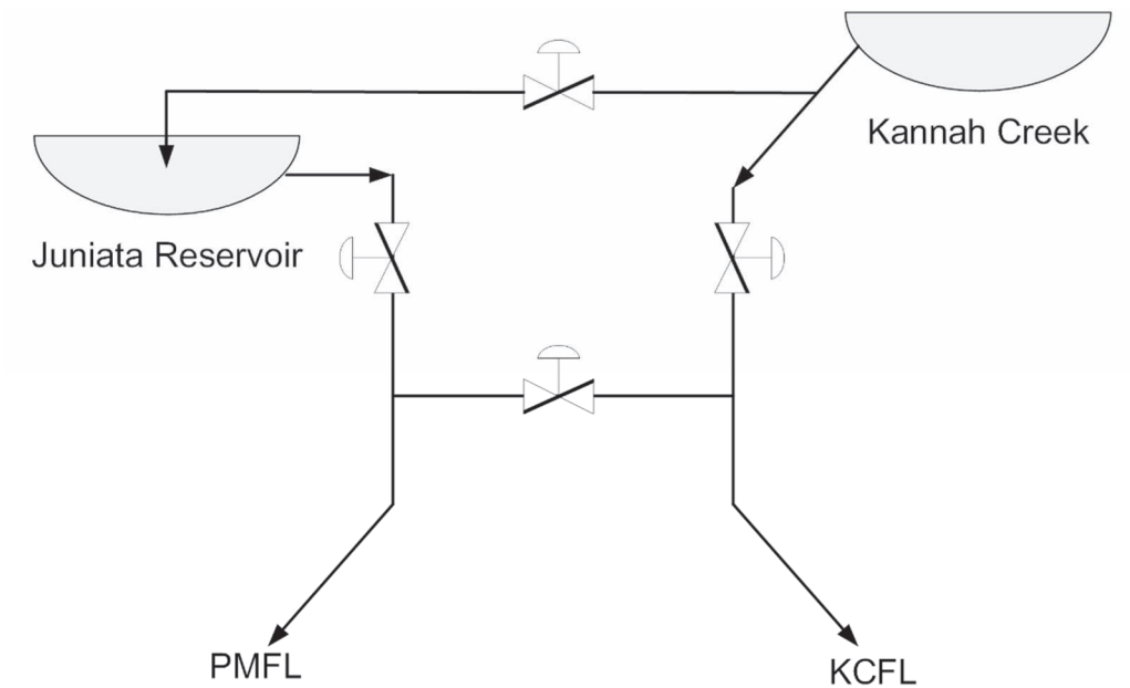
Figure 13: Process Flow Diagram for Juniata Reservoir Interconnection
