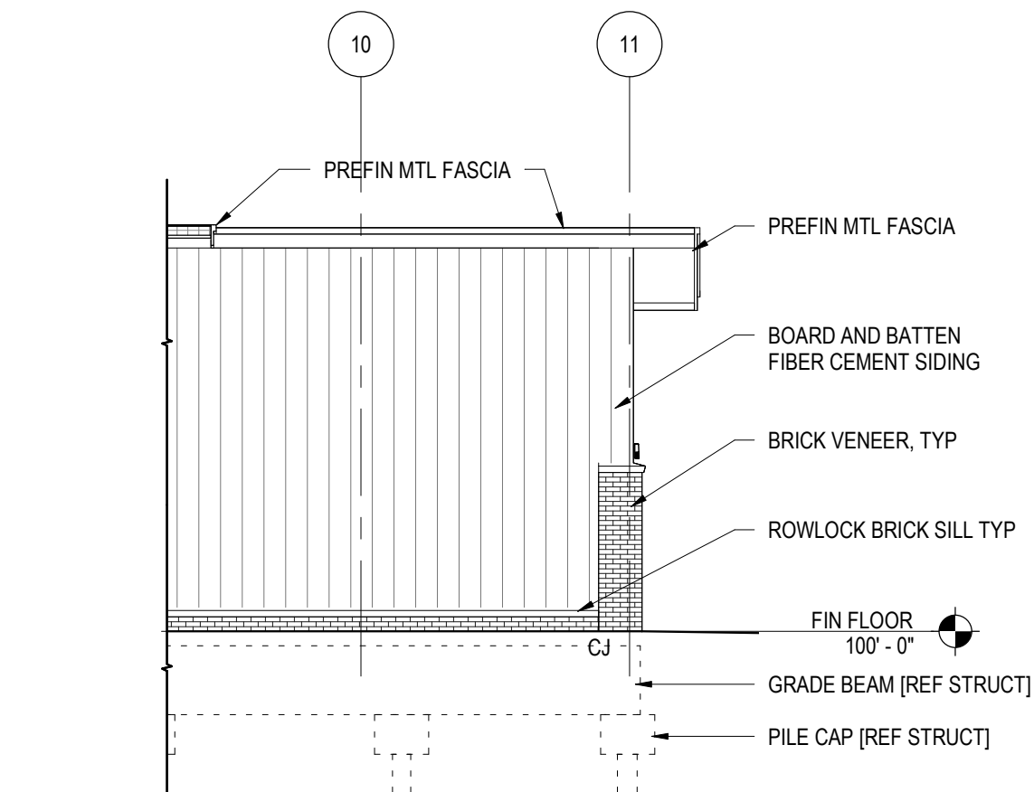
4 SOUTH ELEVATION A2-2 1/8" = 1'-0"
