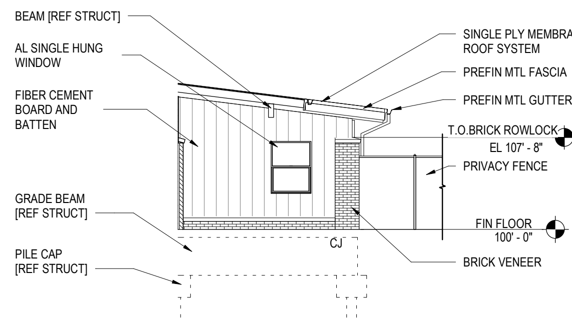
7 WEST ELEVATION A2-2 1/8" = 1'-0"
