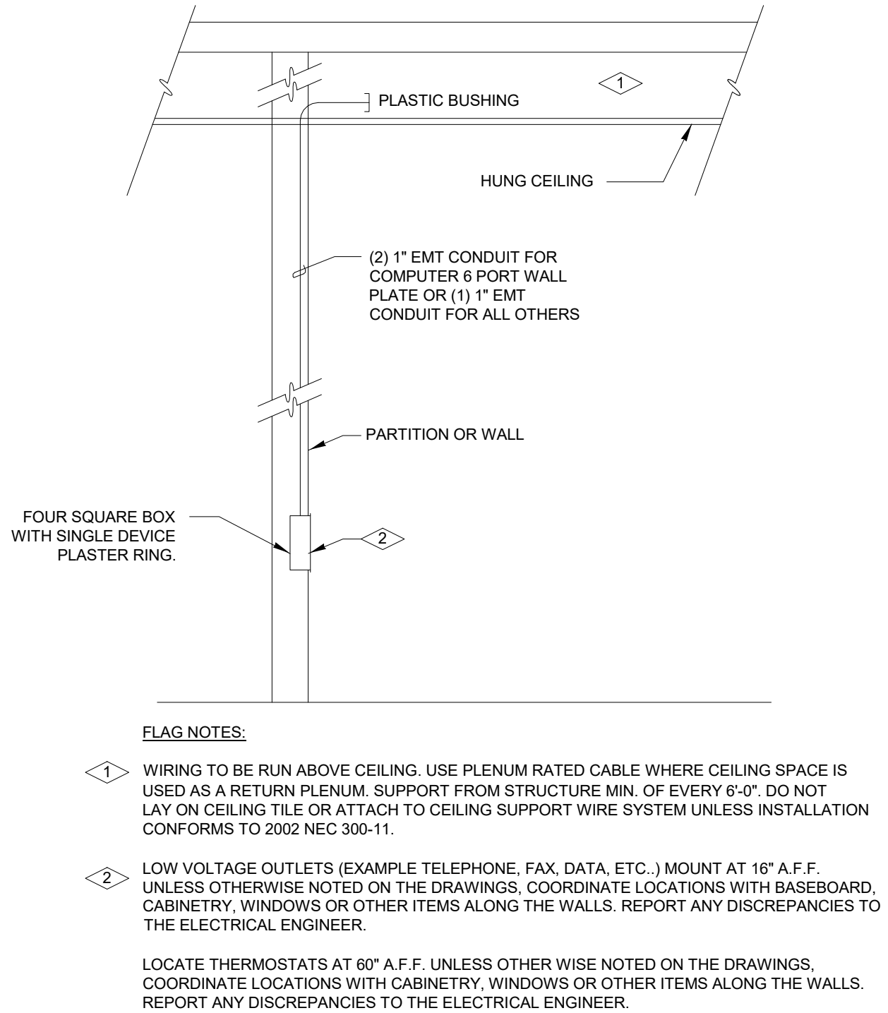
LOW VOLTAGE OUTLET WIRING DETAIL NOT TO SCALE
