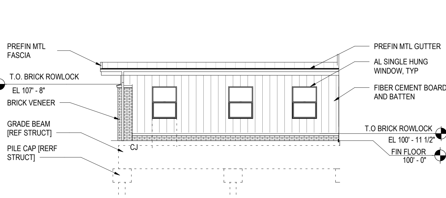
6 NORTH ELEVATION A2-2 1/8" = 1'-0"
