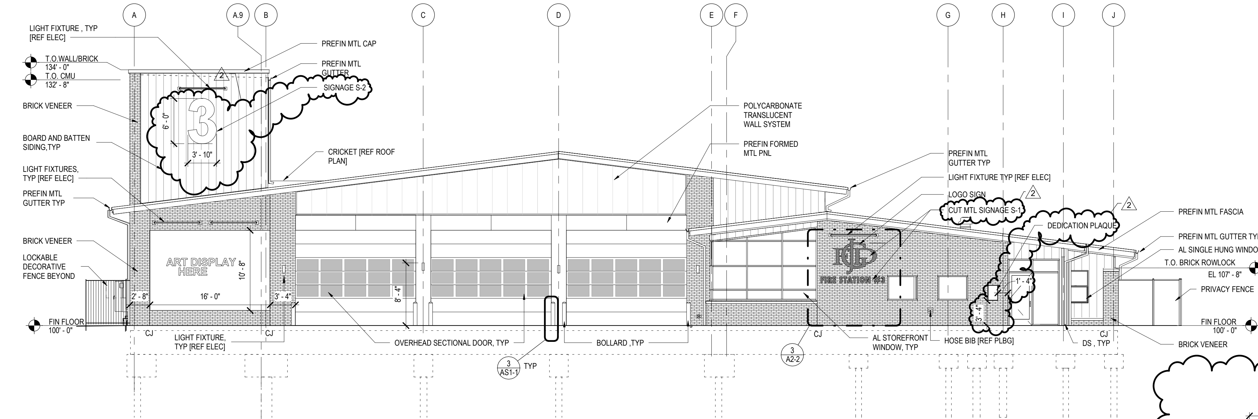
2 WEST ELEVATION A2-2 1/8" = 1'-0"
