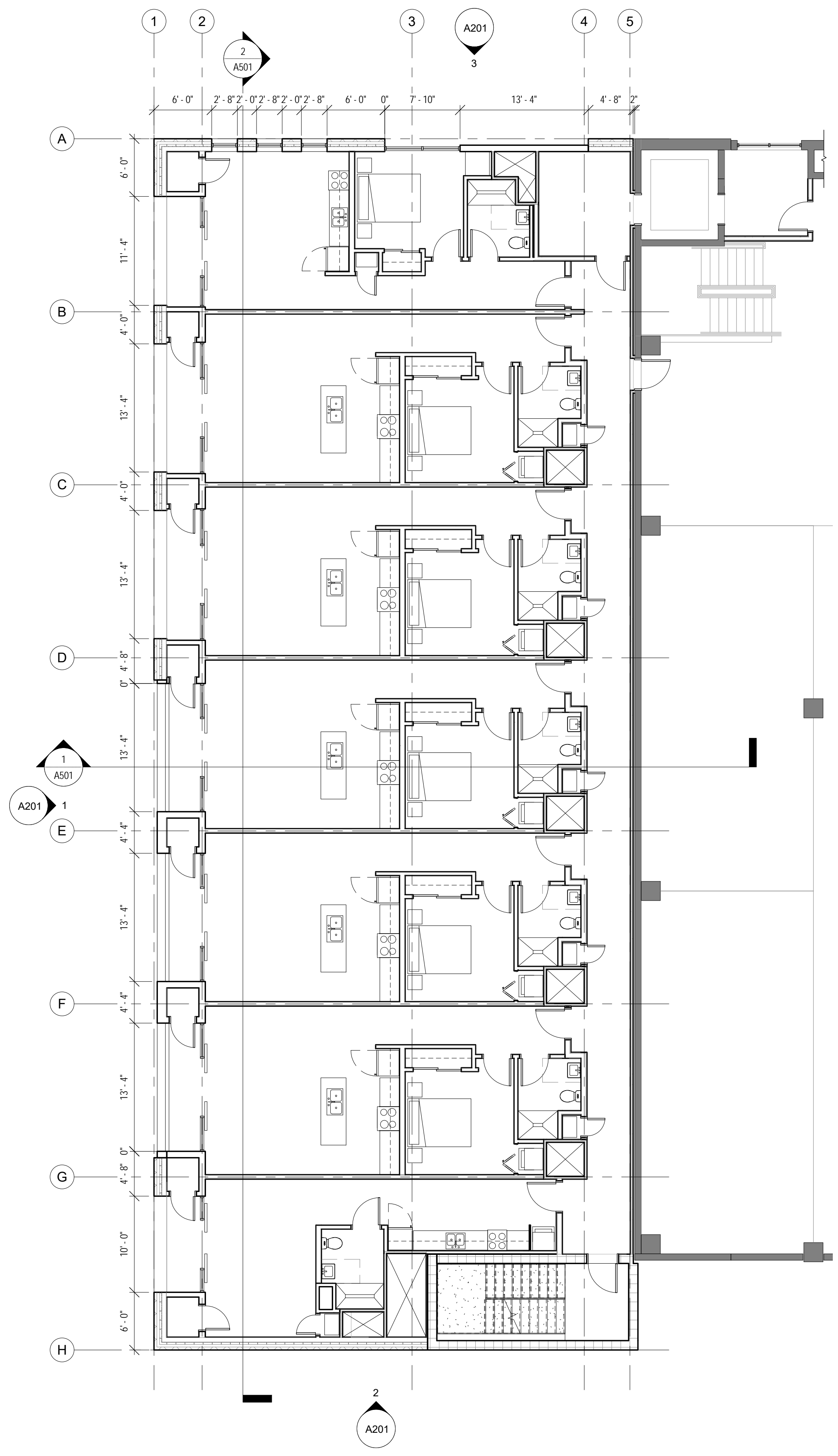
1 3RD FLOOR - CONSTRUCTION PLAN A102
