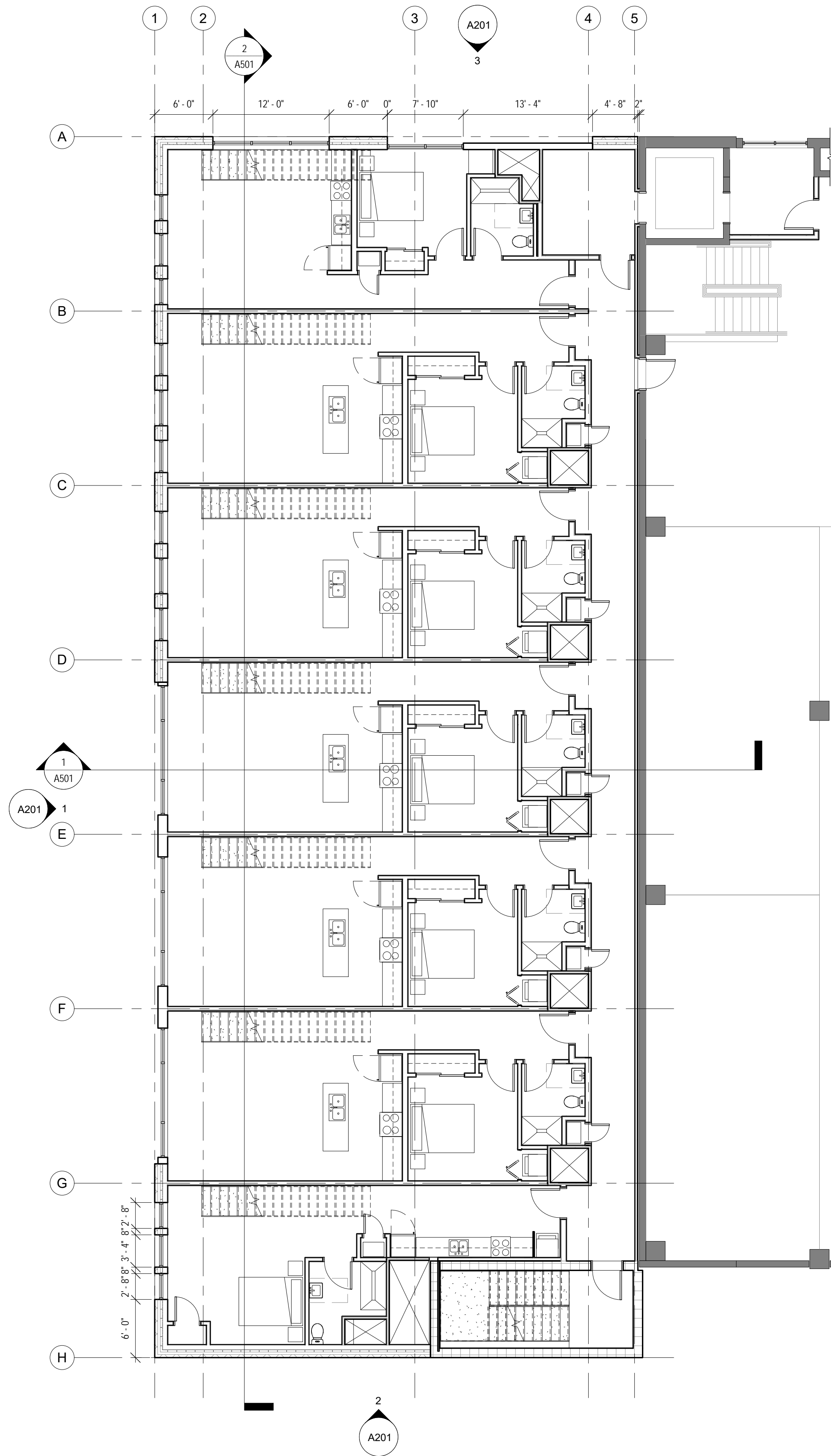
1 4TH FLOOR - CONSTRUCTION PLAN A103
