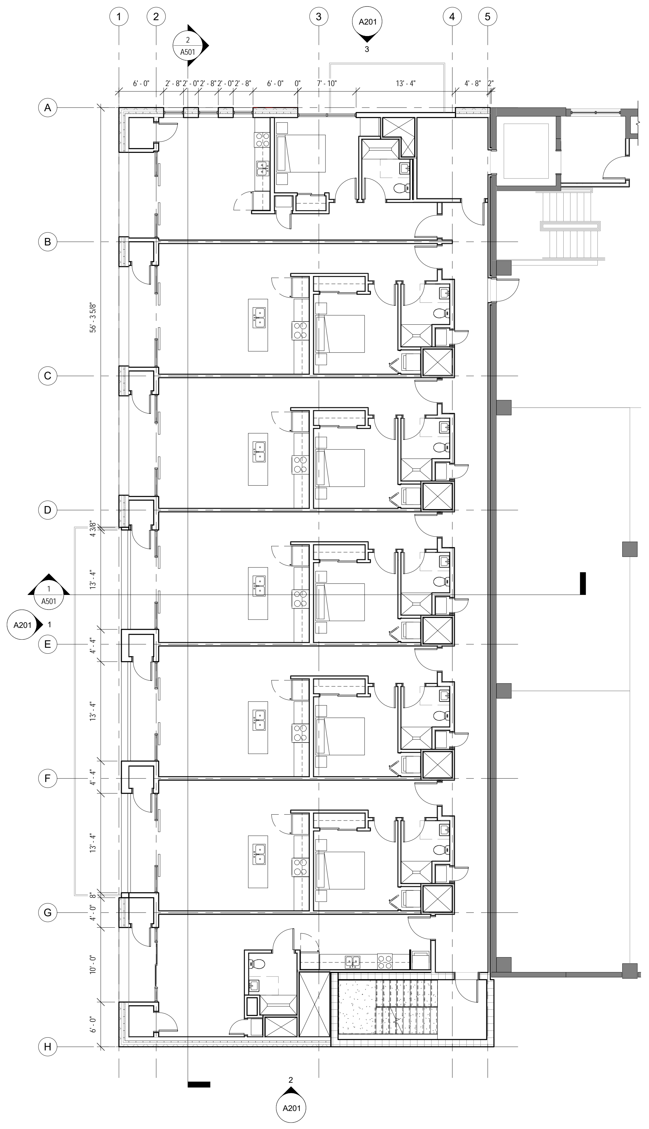
2 2ND FLOOR - CONSTRUCTION PLAN A102
