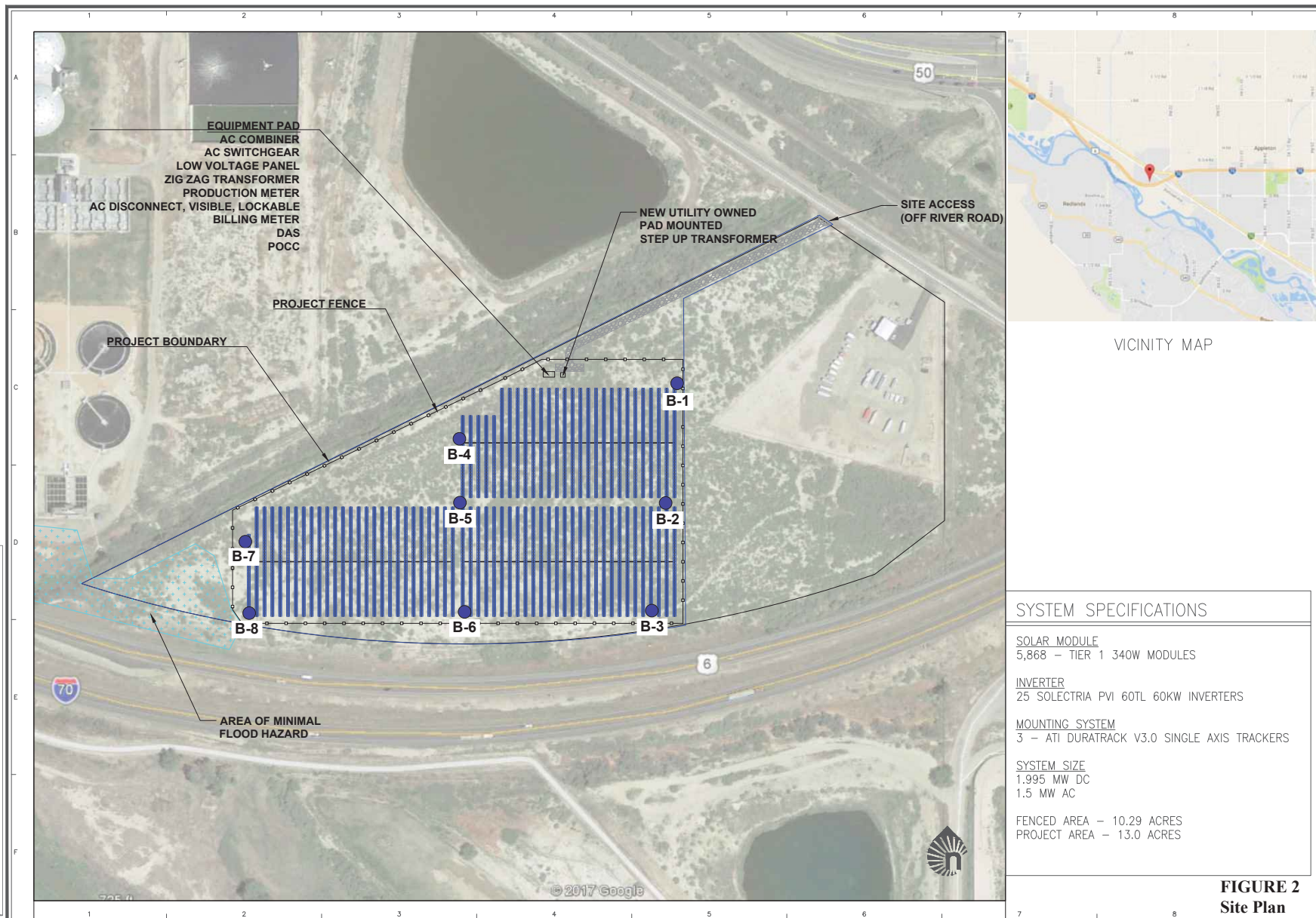
PRELIMINARY SITE PLAN
