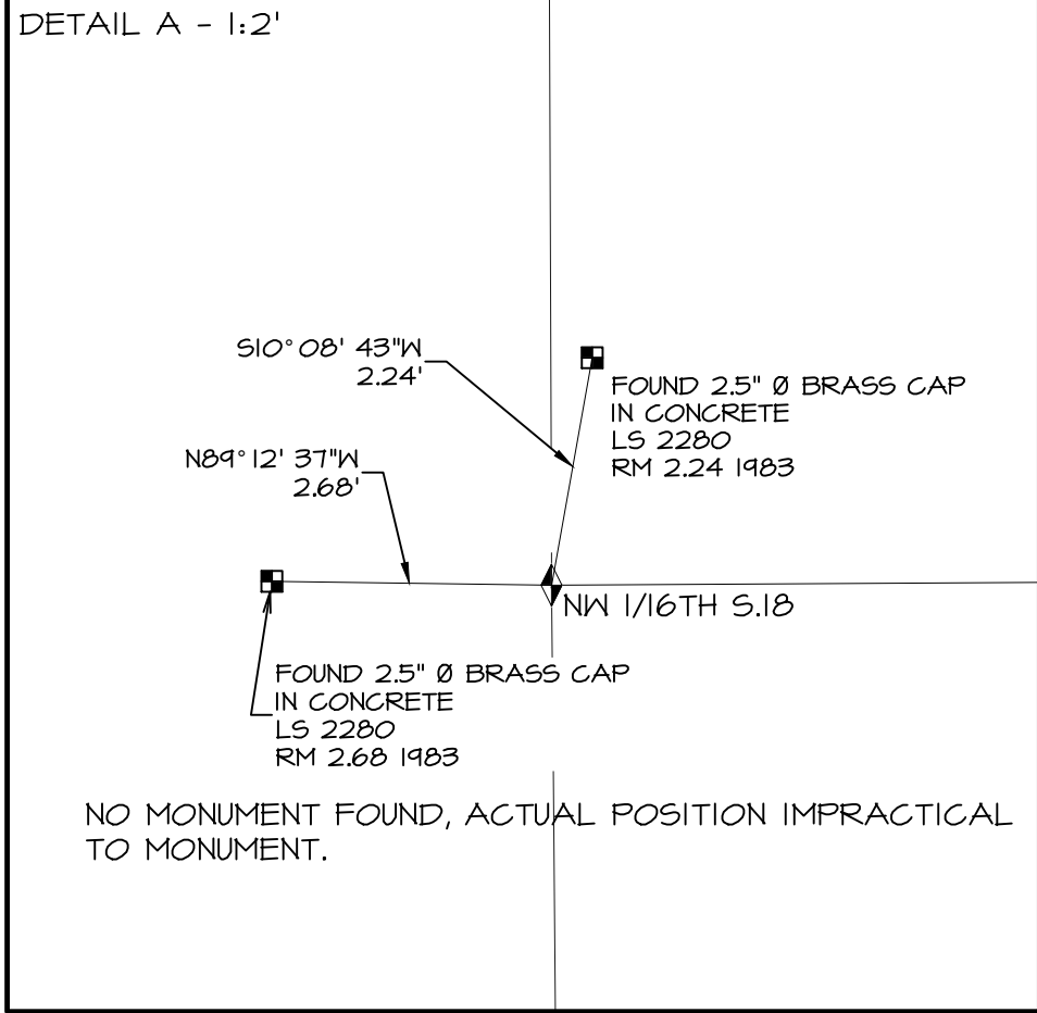
DETAIL A - 1:2'
